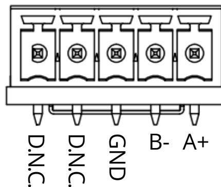
Figure 1: Connection pinout
