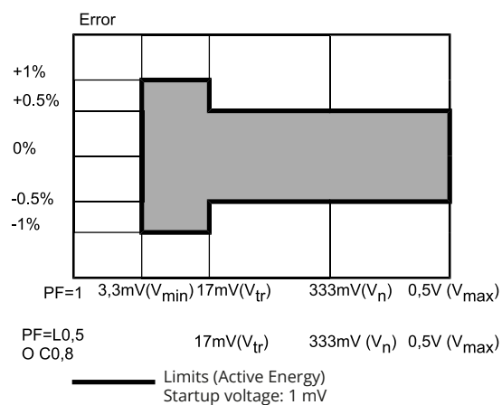
Figure 8: VARh, load-dependent accuracy (CT with current output)
