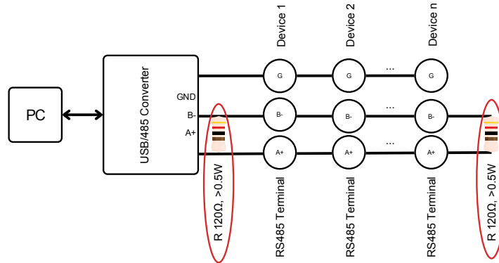
Figure 2: RS485 dynamic bus termination
