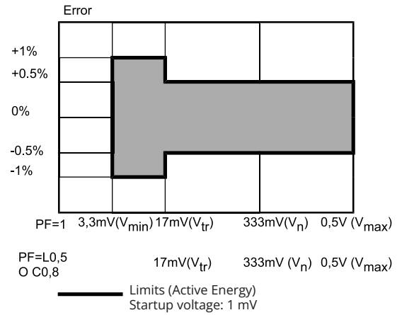
Figure 9: VARh, load-dependent accuracy (CT with current output)
