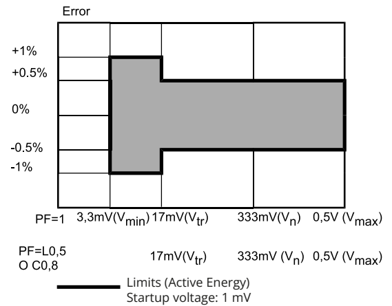
Figure 8: VARh, load-dependent accuracy (CT with current output)
