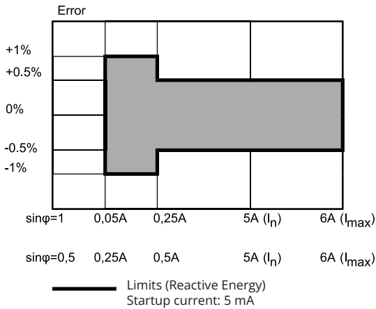
Figure 9: VARh, load-dependent accuracy (CT with voltage output)
