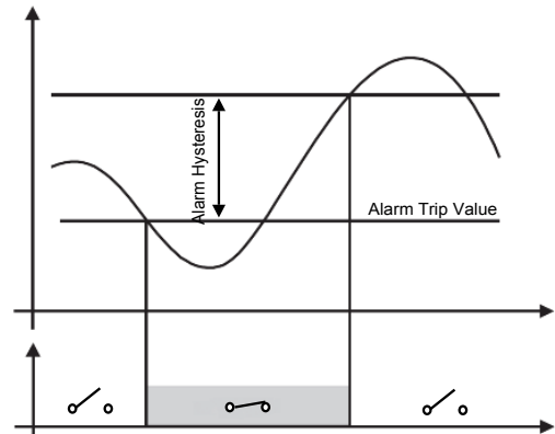
Figure 4: downward: contact normally closed
