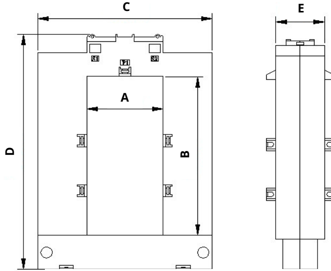
Figure 2: QI-SC-DBPxx-xxx/5 dimensions
