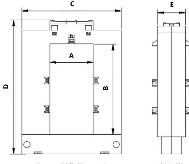
Figure 1: QI-SC-DBPxx-xxx/5 dimensions
