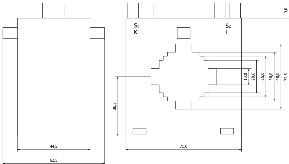
Figure 3: QI-xxx/x-2 dimensions
